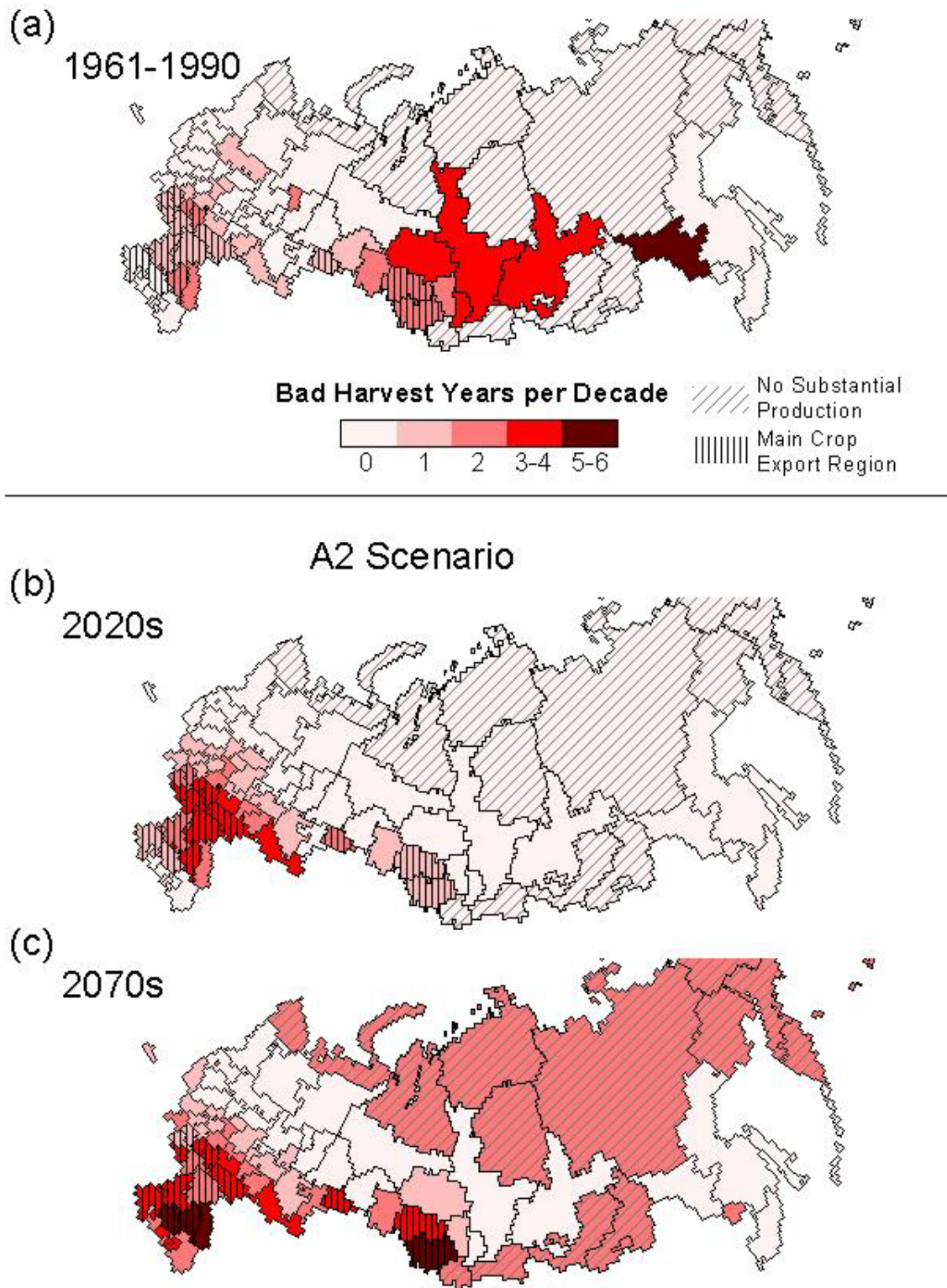
Figure 3: Frequency of bad harvest years computed by the GLASS model for the A2 scenario, with climate scenarios from the HADCM3 model. (a) Frequency under climate normal, (b) 2020s, (c) 2070s.
